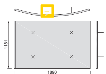
Convex installation
