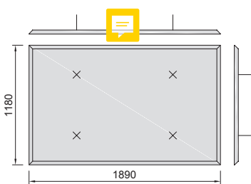
Flat installation
